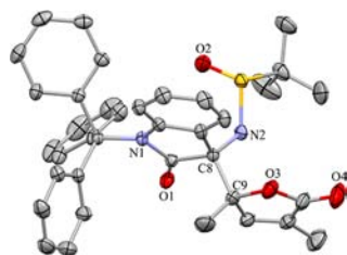
Figure 2. Single crystal X-ray structure of 4f (hydrogen atoms are omitted for clarity).
