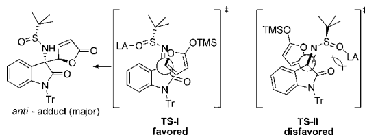
Figure 3. Plausible transition state for the stereochemical outcome.
