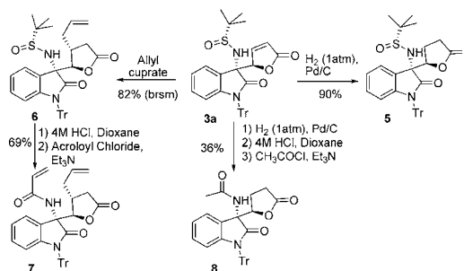
Scheme 1. Transformation of Mannich Adduct 3a
